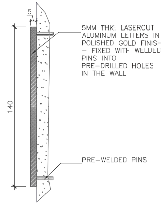
SECTION-A_ SCALE 1:2
